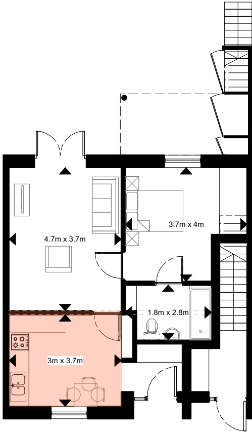
Option 2: Partitioned NSA=51.3m 2 Price estimate: £2500
