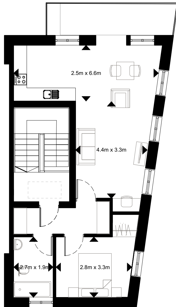
6 Second Floor Plan 1:100 @ A3 NSA=54.8m 2
