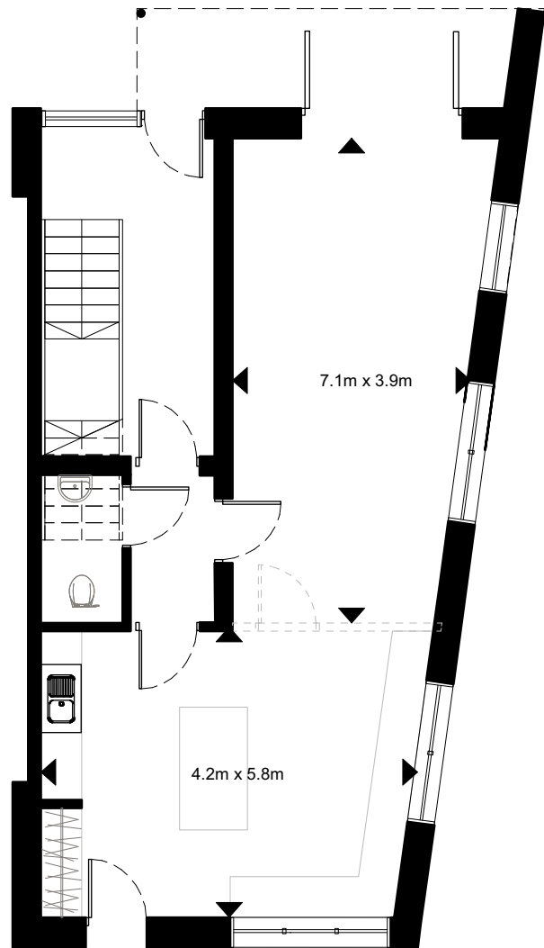
4 Ground Floor Plan 1:100 @ A3 NSA=50.4m 2
